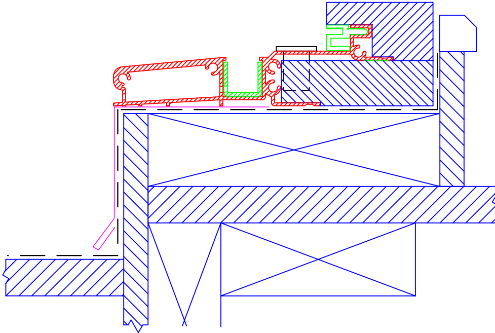
6 9/16" Standard Threshold Flush With Header & Jamb
